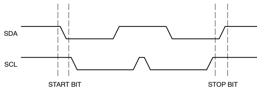
Figure 4. Start/Stop Timing
