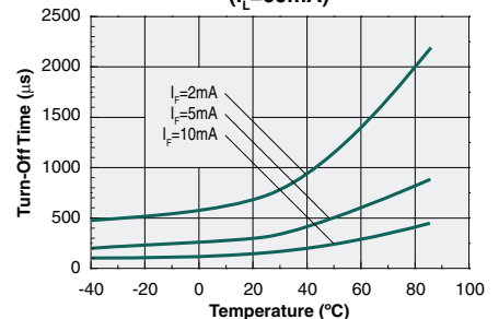
Typical Turn-Off Time vs. Temperature ( I_L=60\text{mA} )
