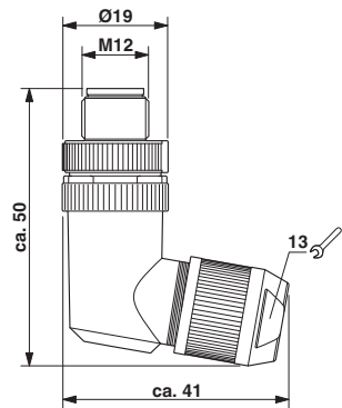
Dimensional drawing
