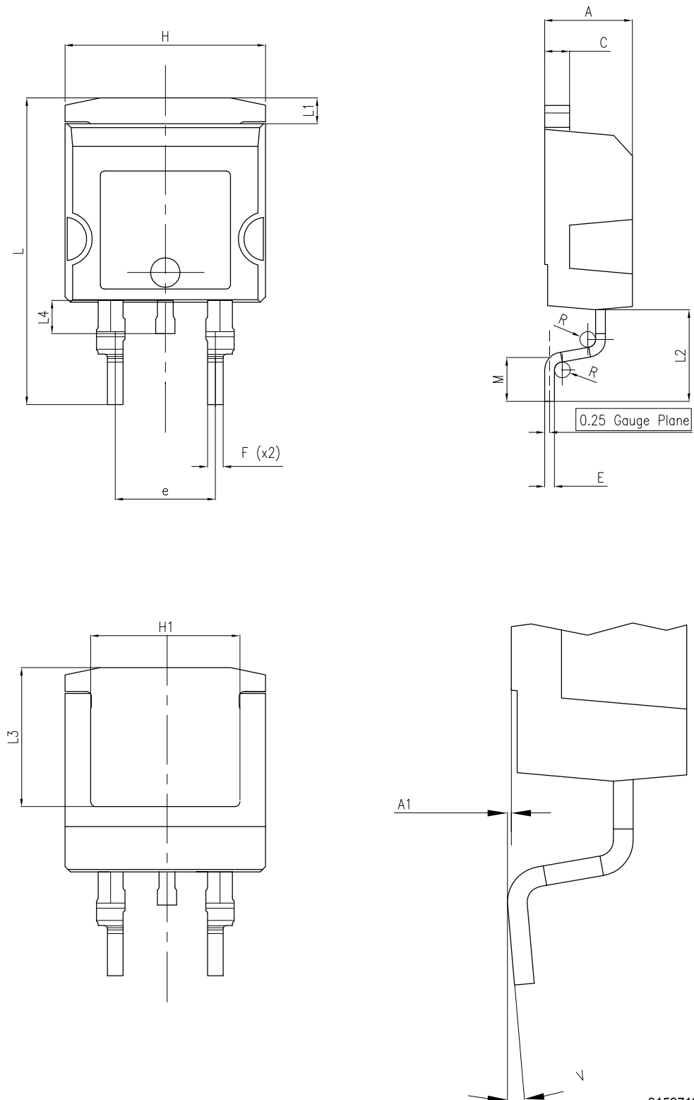
Figure 19. H 2 PAK-2 package outline
