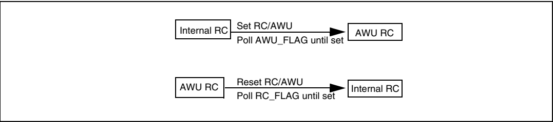
Figure 9. Clock switching
