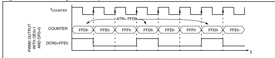
Figure 35. PWM signal example
