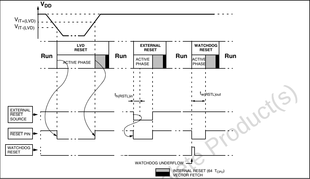
Figure 13. Reset sequences
