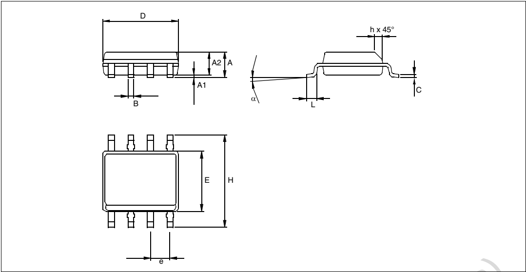
Figure 66. 8-pin plastic small outline package, 150-mil width package outline
