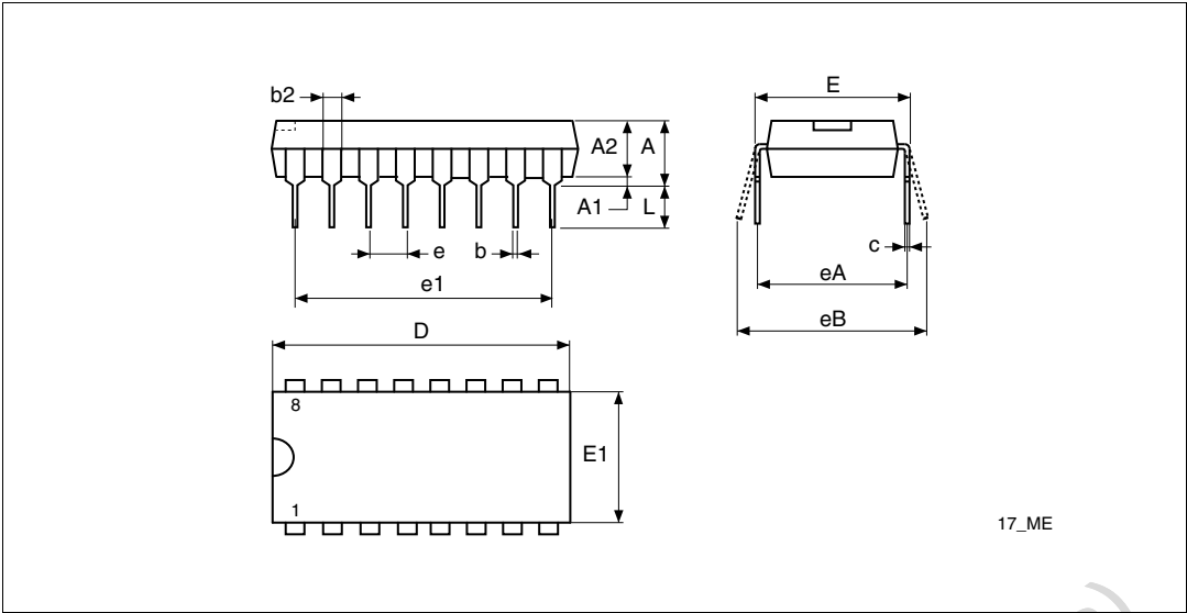
Figure 68. 16-pin plastic dual in-line package, 300-mil width, package outline
