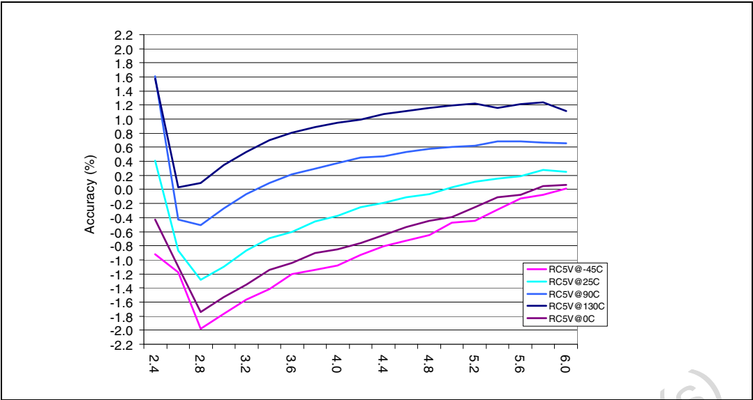
Figure 40. Typical accuracy with RCCR=RCCR0 vs V_{DD} = 2.4-6.0 V and temperature
