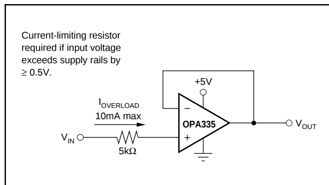
FIGURE 1. Input Current Protection.
