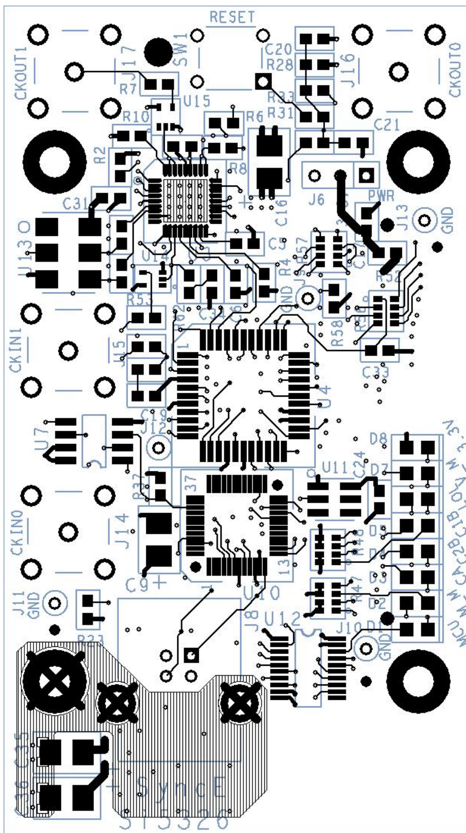
Figure 10. Top Layer
