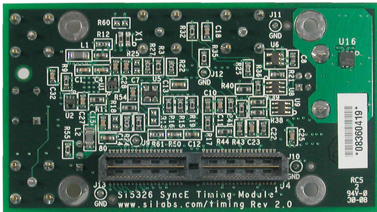
Figure 2. Si5326-VTSS-EVB Bottom
