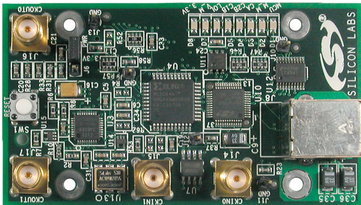
Figure 1. Si5326-VTSS-EVB Top
