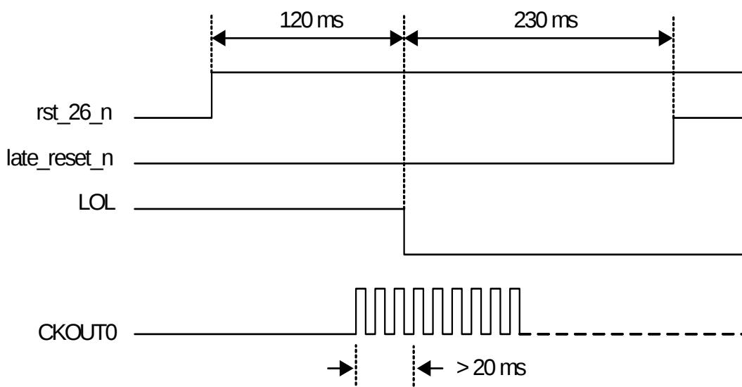
Figure 5. Late Reset Timing
