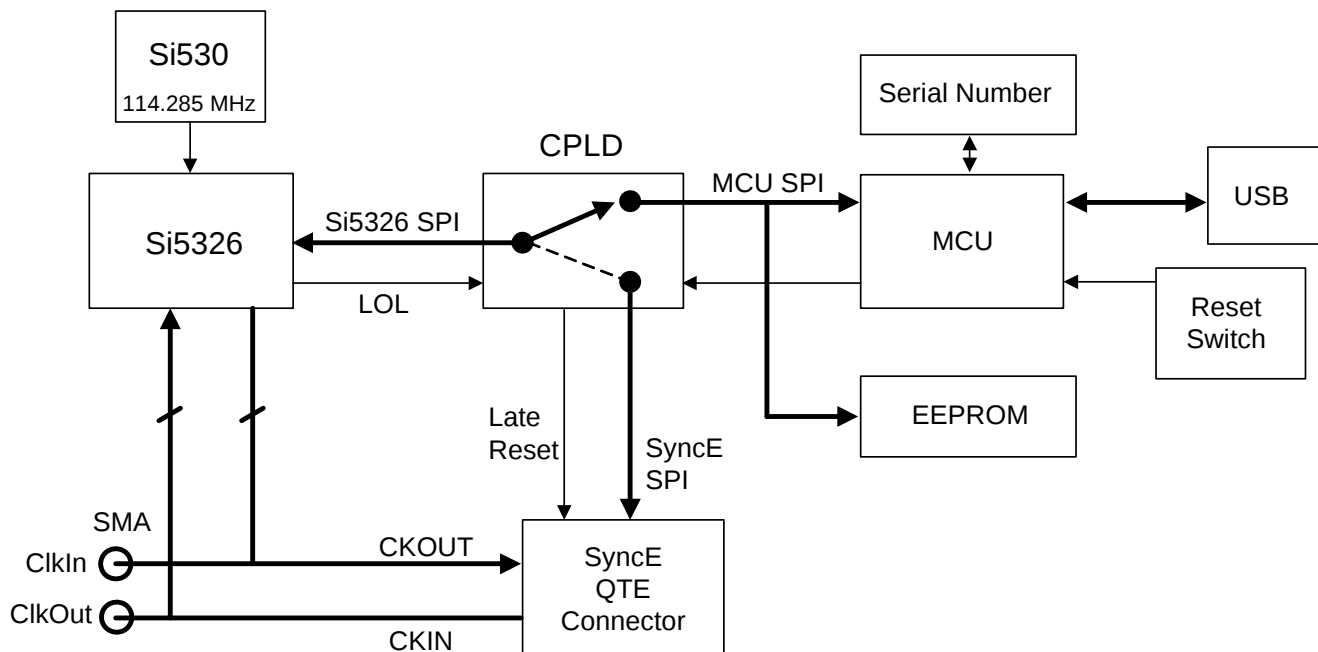
Figure 4. Si5326-VTSS-EVB Block Diagram
