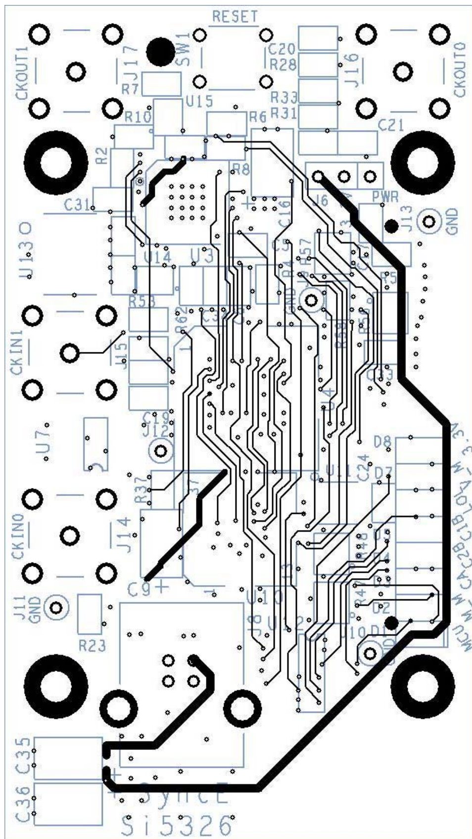
Figure 12. Signal Layer (1 of 2)
