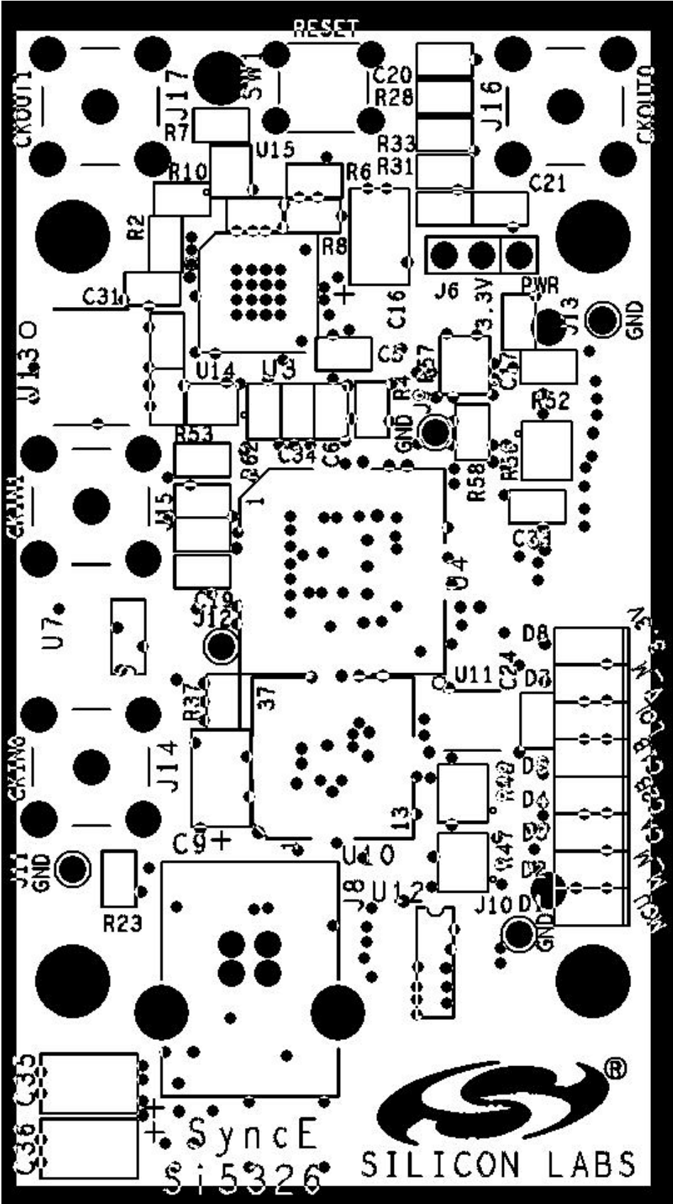
Figure 14. Power Layer
