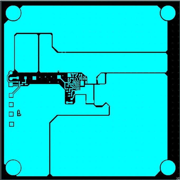
Figure 9: Top Layer
