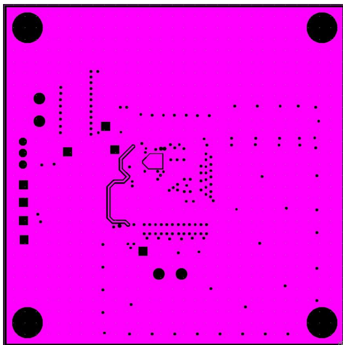
Figure 12: Layer 3
