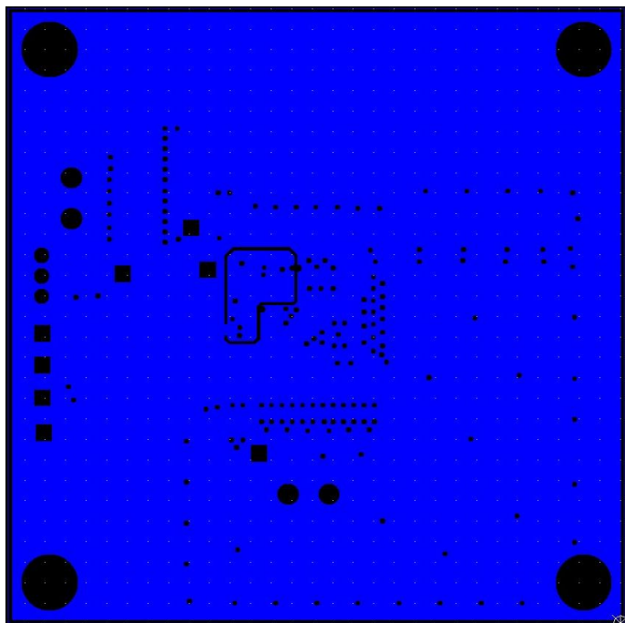
Figure 11: Layer 2
