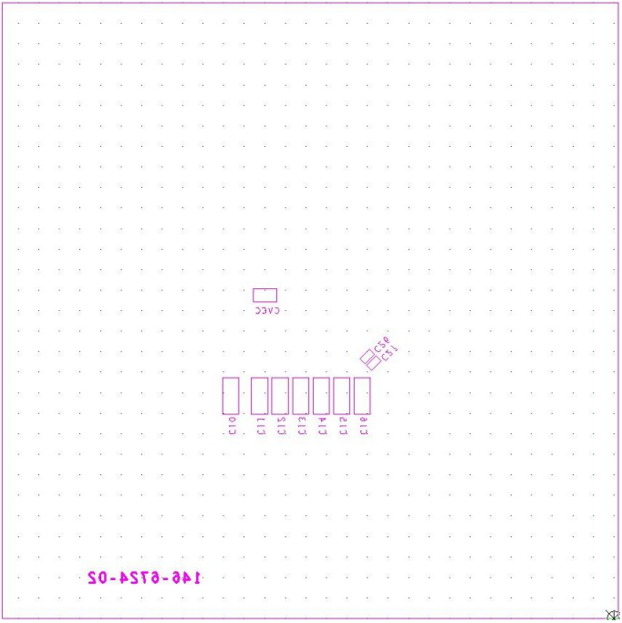
Figure 8: Assembly Bottom
