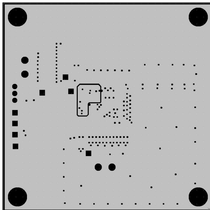
Figure 14: Layer 5
