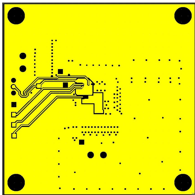
Figure 13: Layer 4
