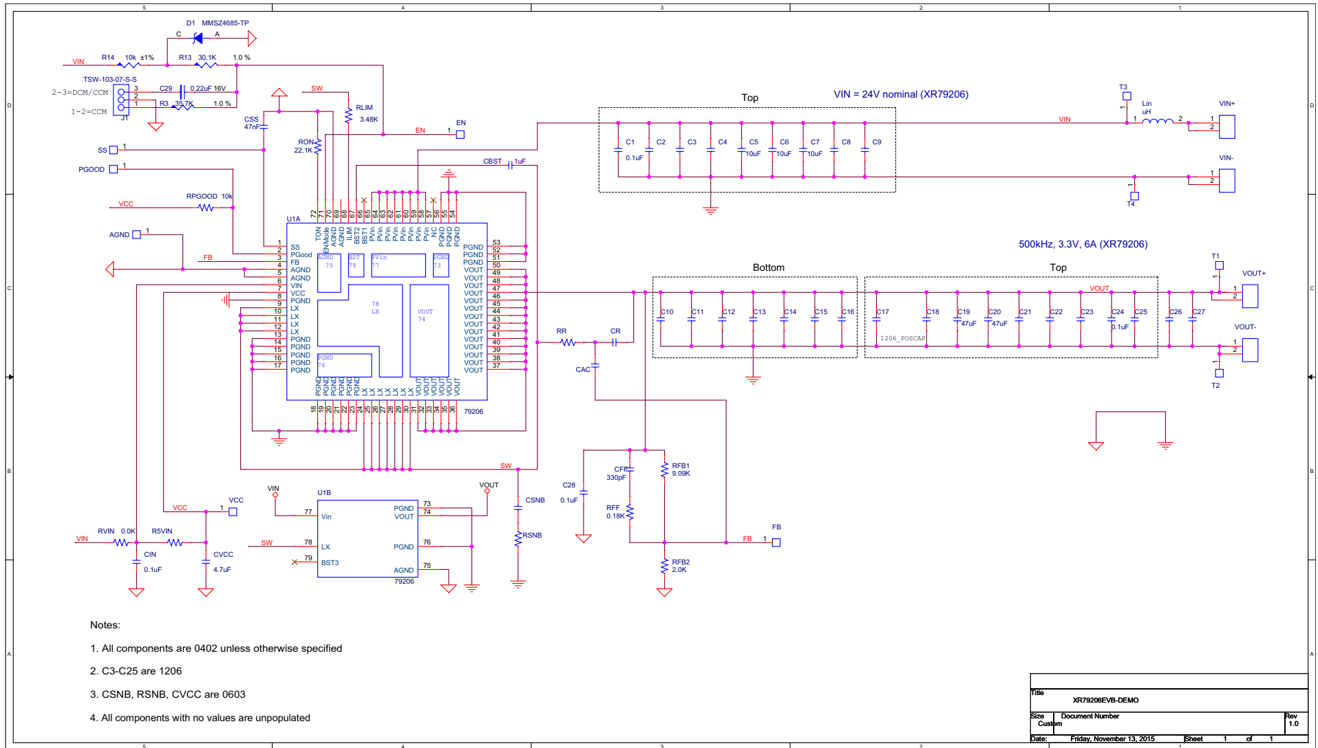
Figure 6: XR79206EVB Schematic
