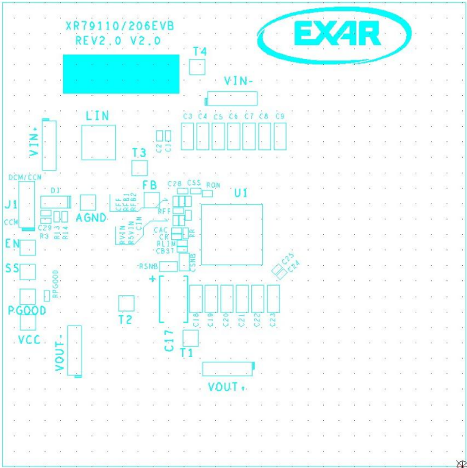
Figure 7: Assembly Top
