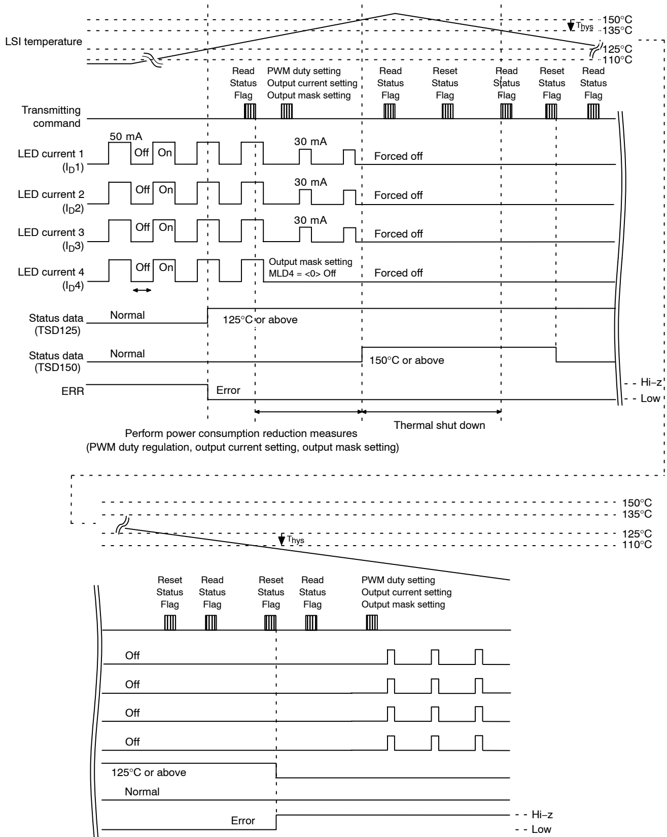
Figure 21. Sequence of the Thermal Shut Down Operating
