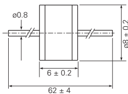
Axial Leads (GTCA28-XXXM-R0X)
