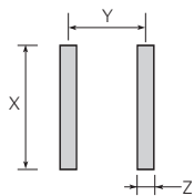
Pad Layout - Surface-mount Devices (GTCS28-XXXM-R05, R10 & R20)
