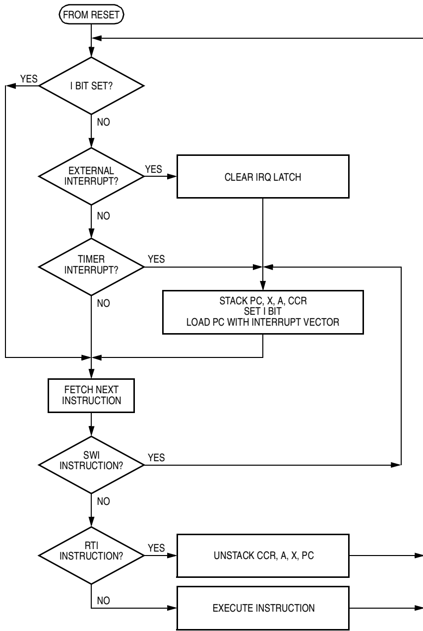
Figure 4-7. Interrupt Flowchart
