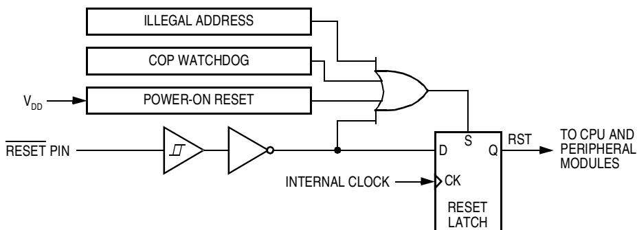
Figure 4-1. Reset Sources
