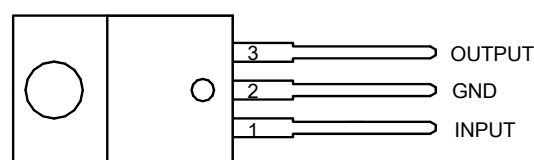
TO-220-3 (Option 2)
