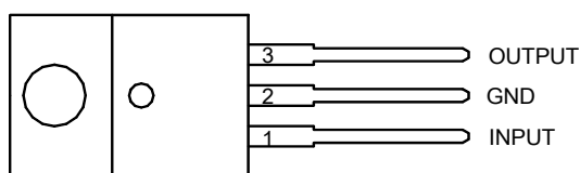
TO-220-3 (Option 1)
