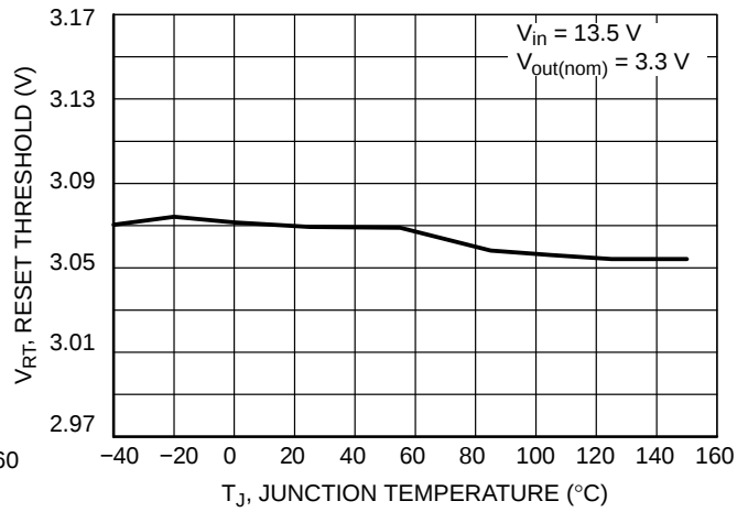
Figure 23. Reset Threshold vs. Junction Temperature
