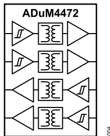
Figure 4. ADuM4472
