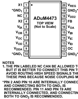
Figure 11. ADuM4473 Pin Configuration
