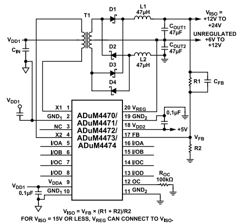
Figure 49. Doubling Power Supply
