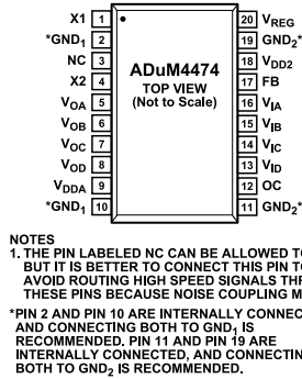
Figure 12. ADuM4474 Pin Configuration
