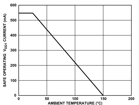
Figure 7. Thermal Derating Curve, Dependence of Safety Limiting Values on Case Temperature, per DIN EN IEC 60747-17 (VDE 0884-17)
