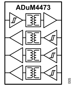
Figure 5. ADuM4473
