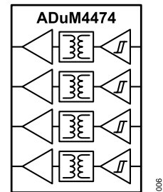
Figure 6. ADuM4474
