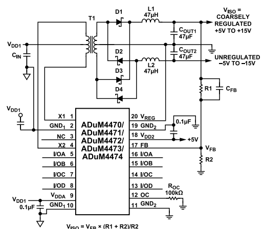
Figure 50. Positive and Unregulated Negative Supply
