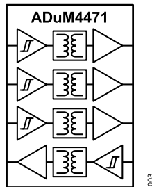
Figure 3. ADuM4471
