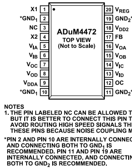
Figure 10. ADuM4472 Pin Configuration
