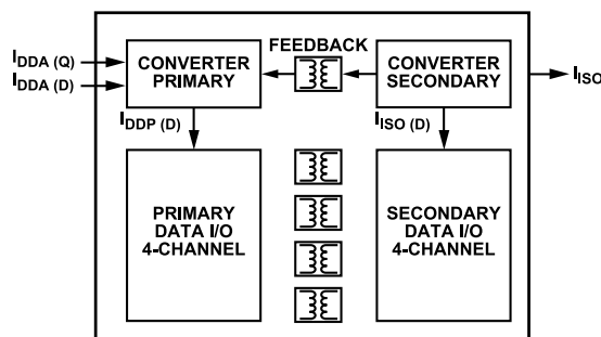
Figure 55. Power Consumption Within the ADuM447x
