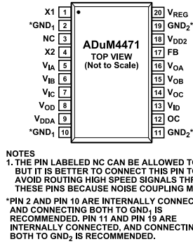
Figure 9. ADuM4471 Pin Configuration
