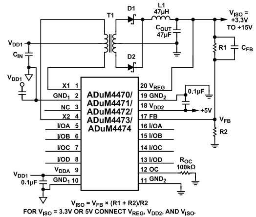
Figure 48. Single Power Supply
