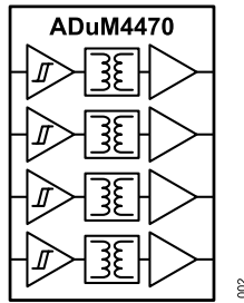
Figure 2. ADuM4470
