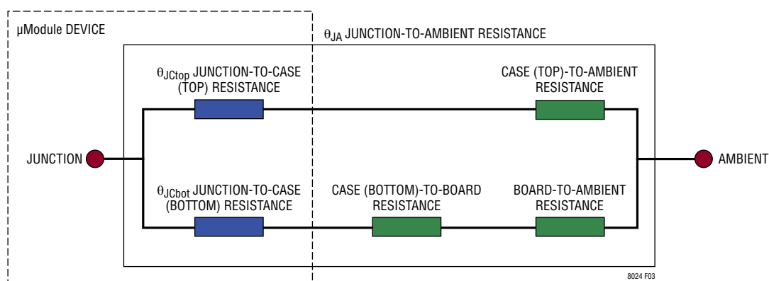
Figure 3. Graphical Approximation of the Thermal Coefficients, Including JESD51-12 Terms
