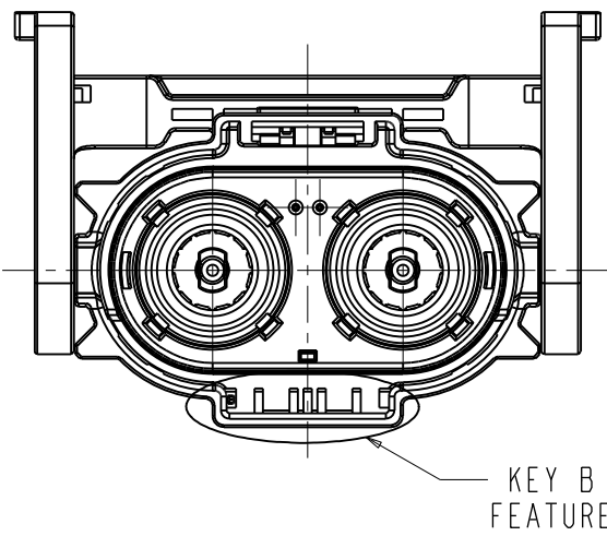
HVSL1400062BXXX
