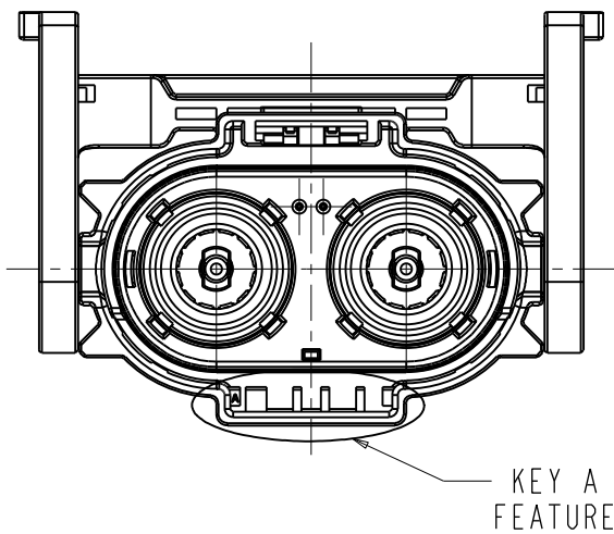
HVSL1400062AXXX
