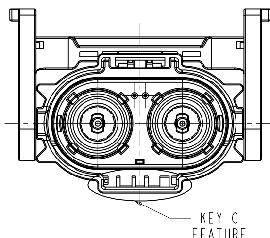
HVSL1400062CXXX
