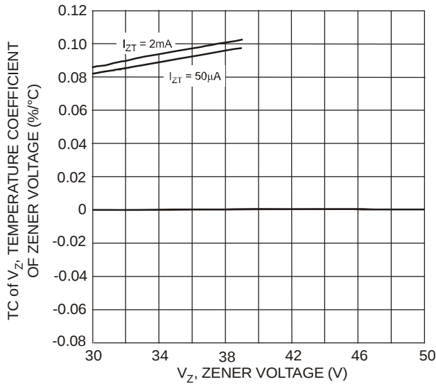
Fig. 20 Typical Temperature Coefficient of Zener Voltage vs. Zener Voltage, DDZX9713S - DDZX9716S
