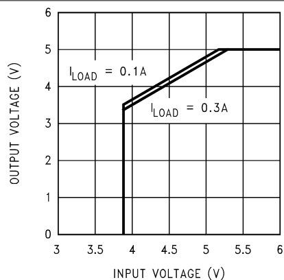
Figure 7-14. Dropout Voltage, 5-V Version
