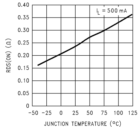
Figure 7-4. Drain-to-Source Resistance
