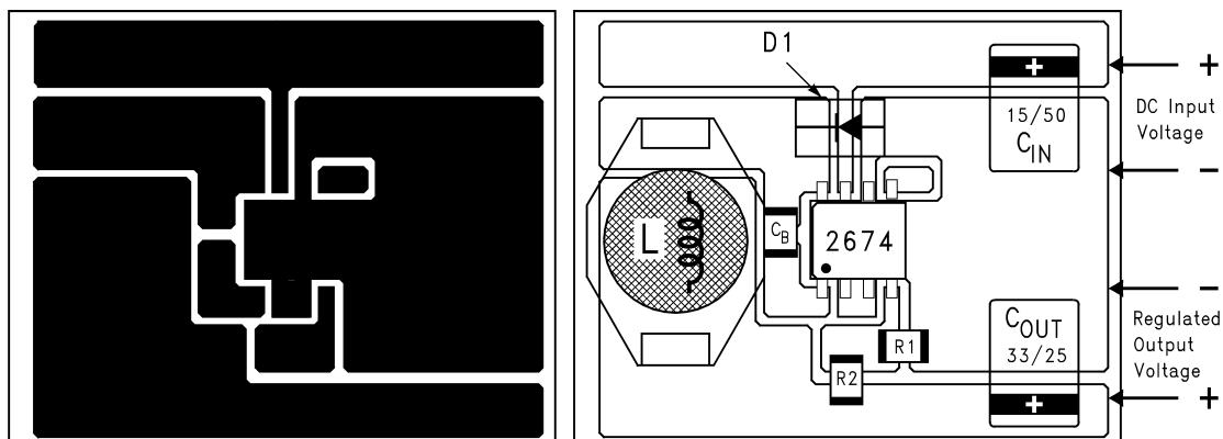
Figure 9-14. Typical Surface-Mount PCB Layout, Fixed Output (4x Size)
