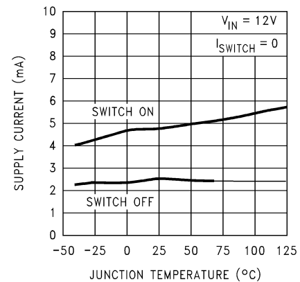
Figure 7-6. Operating Quiescent Current
