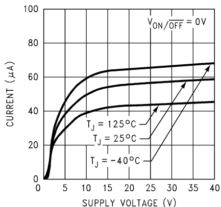
Figure 7-7. Standby Quiescent Current
