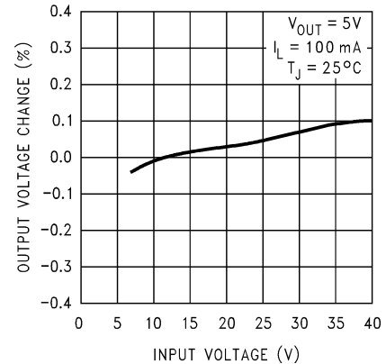
Figure 7-2. Line Regulation
