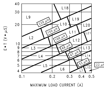
Figure 9-13. LM2674, Adjustable Version
