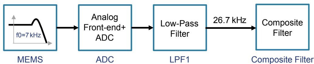
Figure 11. Filtering chain
