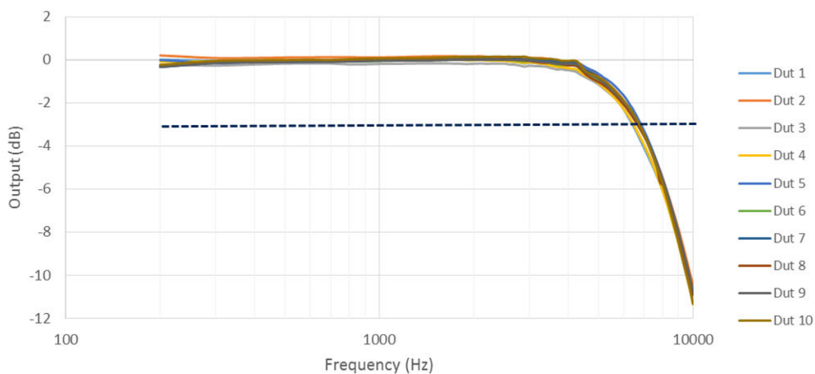
Figure 15. Frequency response - X-axis
