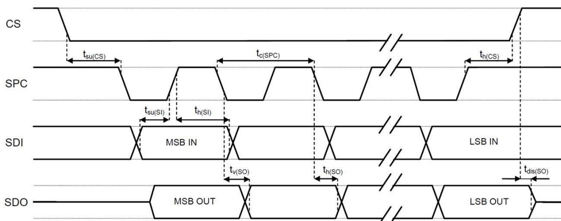
Figure 2. SPI slave timing diagram
