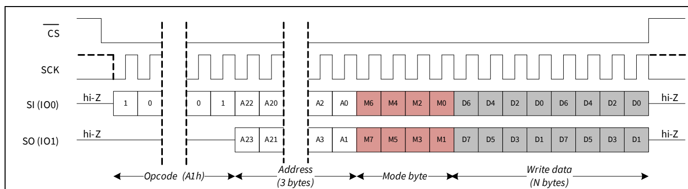
Figure 48 Dual I/O write (DIOW)
