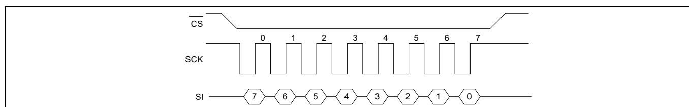
Figure 5 SPI mode 3
