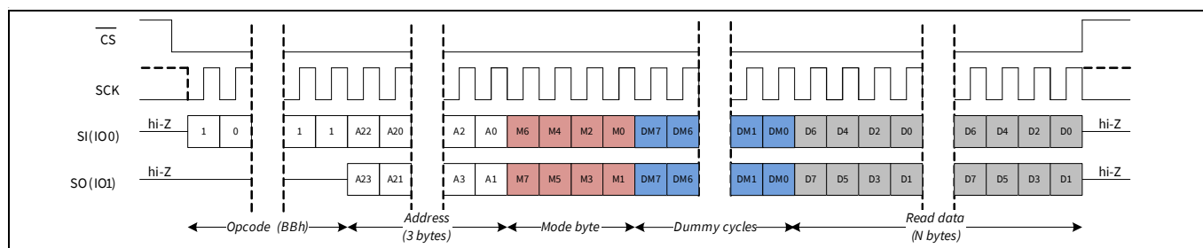
Figure 60 Double I/O read (DIOR)
