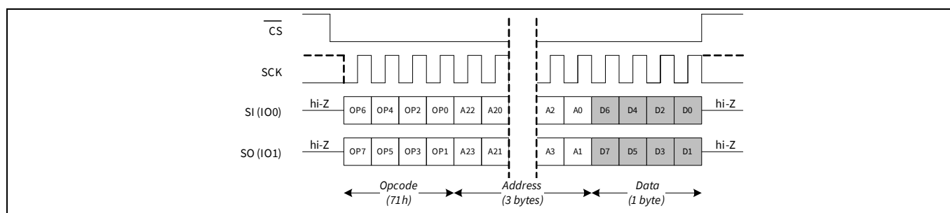
Figure 34 Write Any Register (WRAR) in DPI mode
