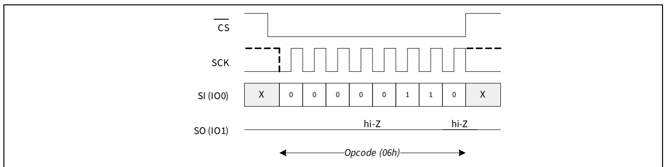
Figure 6 WREN bus configuration in SPI mode
