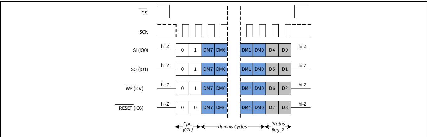
Figure 19 Read SR2 (RDSR2) in DPI mode
