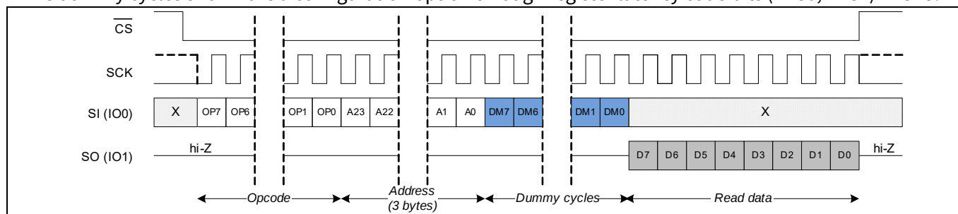
Figure 36 Read Any Register (RDAR) in SPI mode
