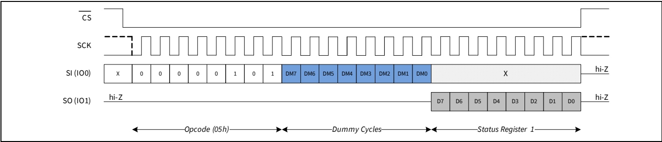
Figure 15 Read SR1 (RDSR1) in SPI mode
