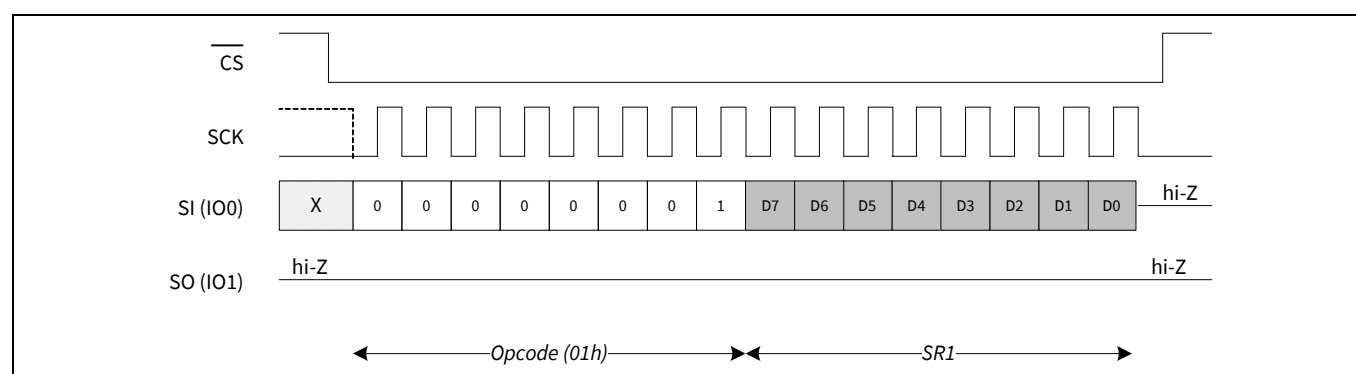
Figure 12 WRSR in SPI mode (WREN not shown)
