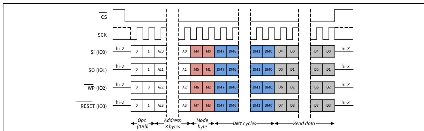
Figure 57 FAST_READ in QPI mode
