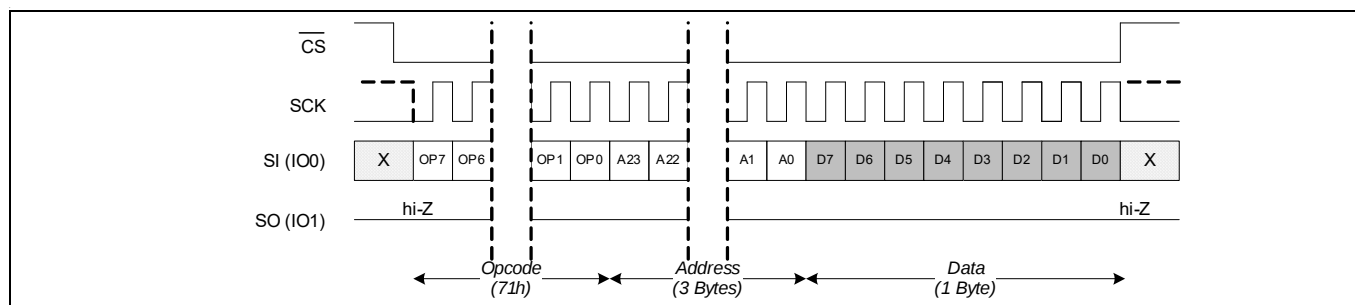
Figure 33 Write Any Register (WRAR) in SPI mode
