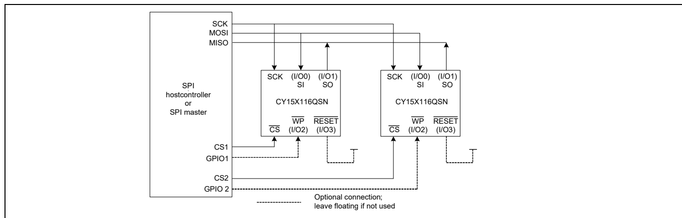
Figure 2 System configuration with SPI port
