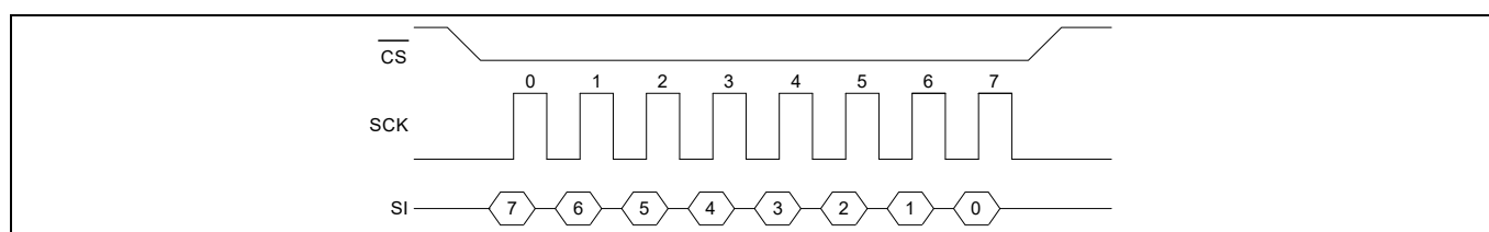
Figure 4 SPI mode 0
