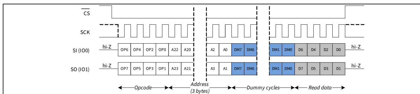
Figure 37 Read Any Register (RDAR) in DPI mode
