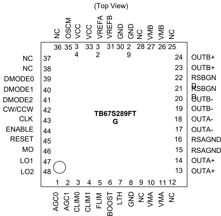
Figure 3.1 Pin Assignments
