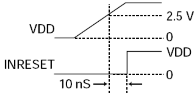
Figure 3: Reset Timing
