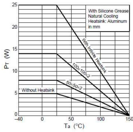
P_T - T_a Characteristics
