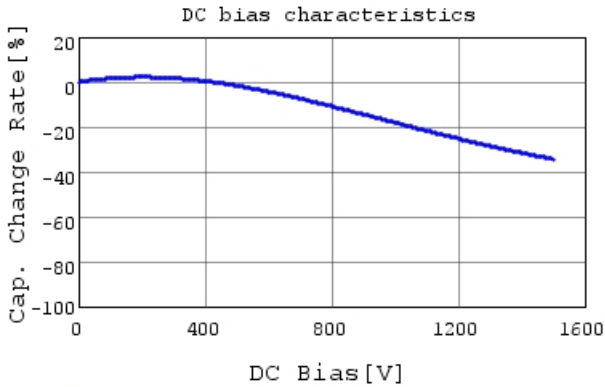
DE2B3SA471KN3AY02F C-DC bias capchange, 20.0
