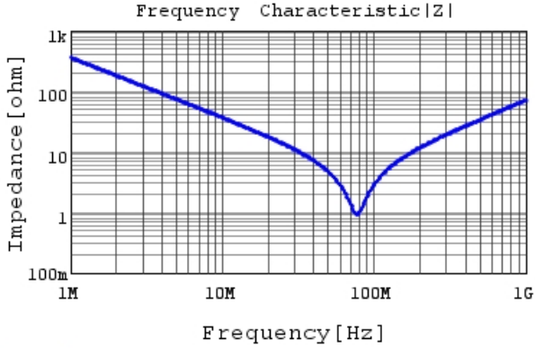
DE2B3SA471KN3AY02F |Z| DCOV, 20degC
