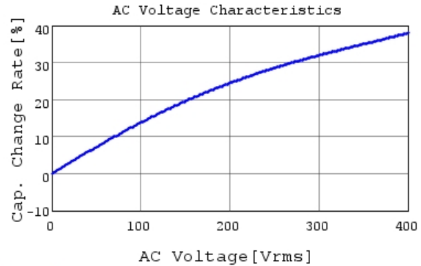
DE2B3SA471KN3AY02F C-AC Voltage capchange, I
