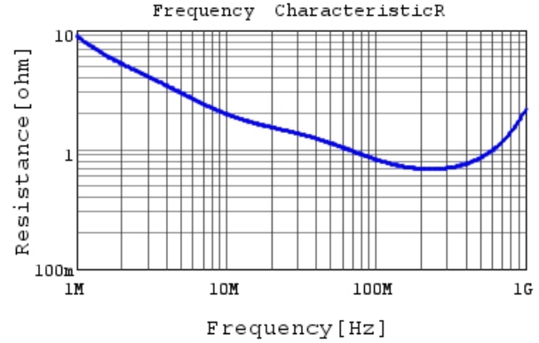
DE2B3SA471KN3AY02F R DCOV, 20degC
