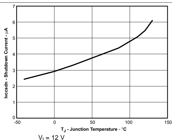
Figure 2. VIN Shutdown Current vs Junction Temperature
