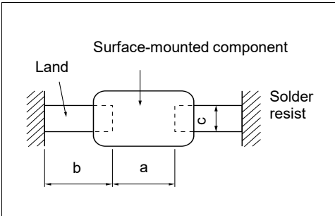
<Recommended land dimensions (example)>
