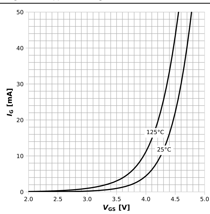
Diagram 14: Typ. transfer gate current characteristic
