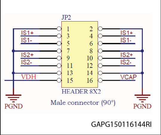
Figure 13. Gate driver board connector: phase signals
