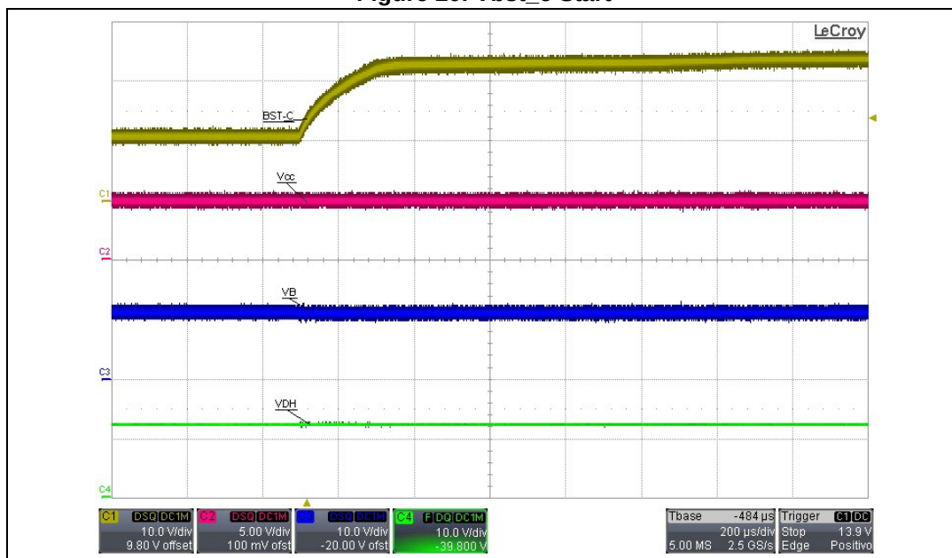
Figure 20. Vbst_c Start
