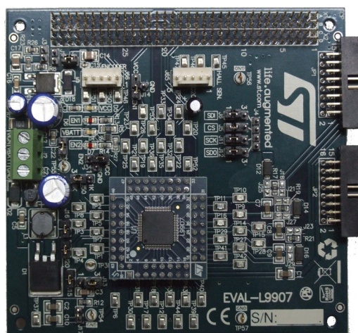
Figure 3. Gate driver board - top view
