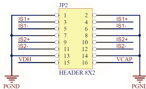
Figure 17. Inverter board connector - phase signals- Male
