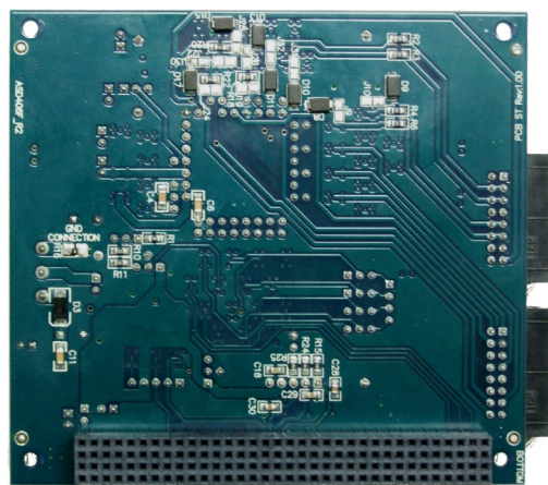
Figure 4. Gate driver board – bottom view
