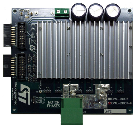
Figure 7. Output Power Board – top view
