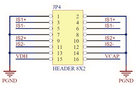
Figure 18. Inverter board connector - phase signals- Female
