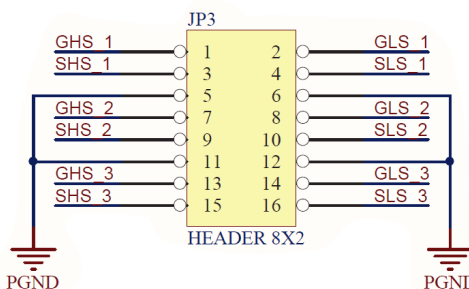
Figure 16. Inverter board connector - control signals- Female
