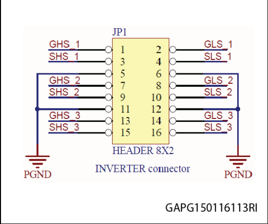
Figure 12. Gate driver board connector: control signals
