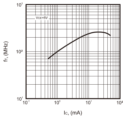
Fig.3 - Transition Frequency
