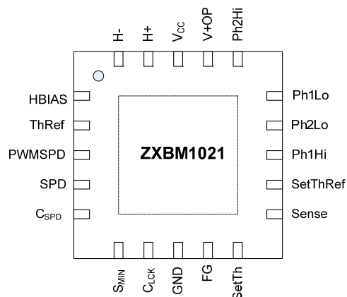
U-QFN4040-20
