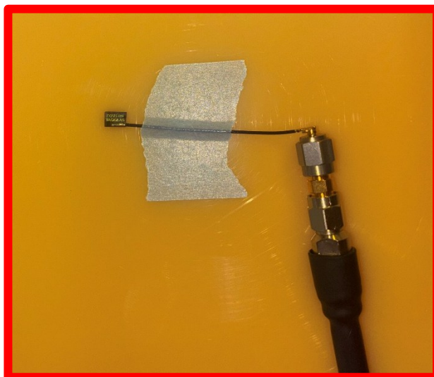
VNA Test Setup on 2mm ABS
