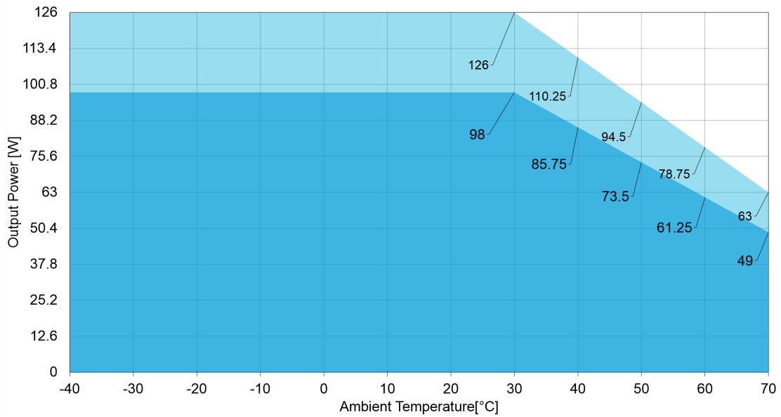
Figure 5. Power Derating of 12 V & 15 V models (Cover kit option)
