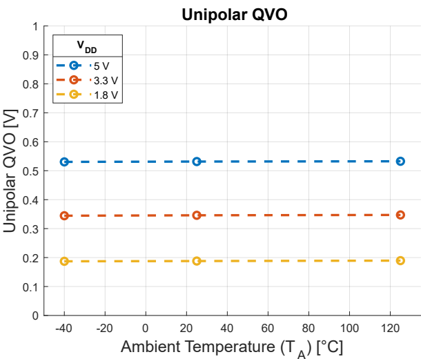
Figure 7: Unipolar QVO
