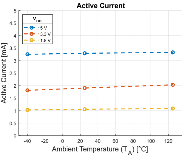
Figure 5: Active Current
