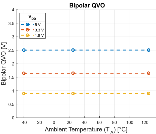
Figure 6: Bipolar QVO
