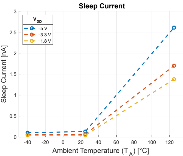
Figure 4: Sleep Current
