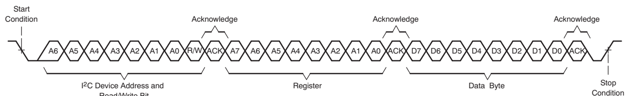
Figure 6. Single-Byte Write Transfer
