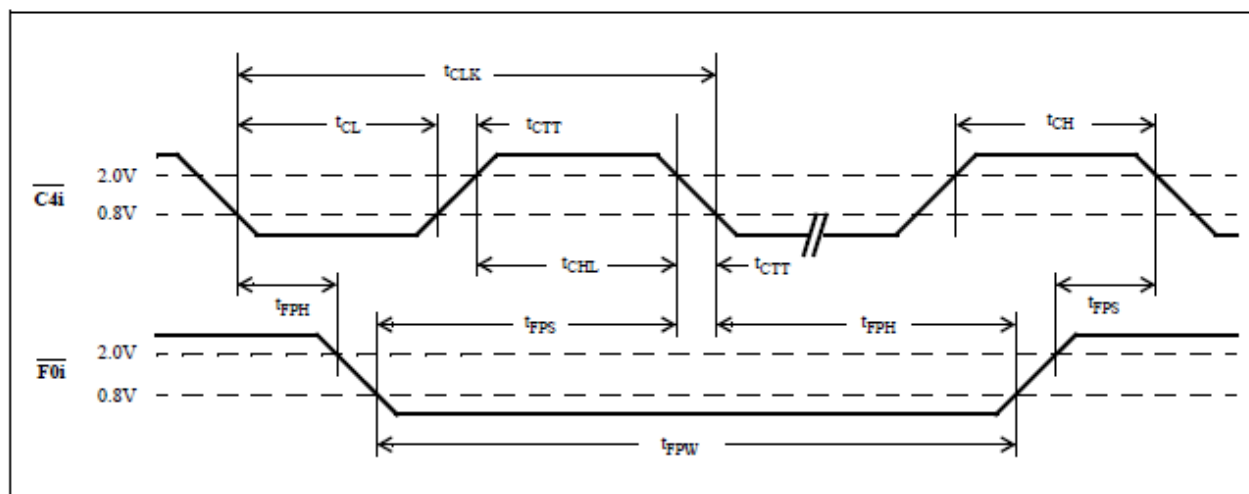
Figure 13 - Clock Timing
