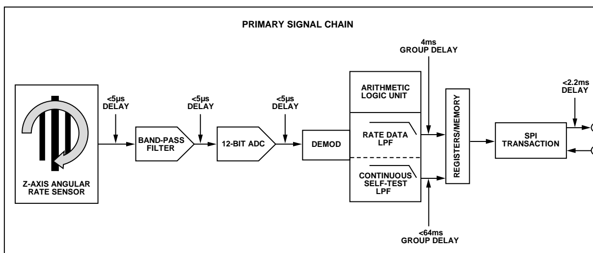
Figure 17. ADXRS810 Primary Signal Chain and Associated Delays
