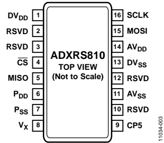
Figure 3. Pin Configuration
