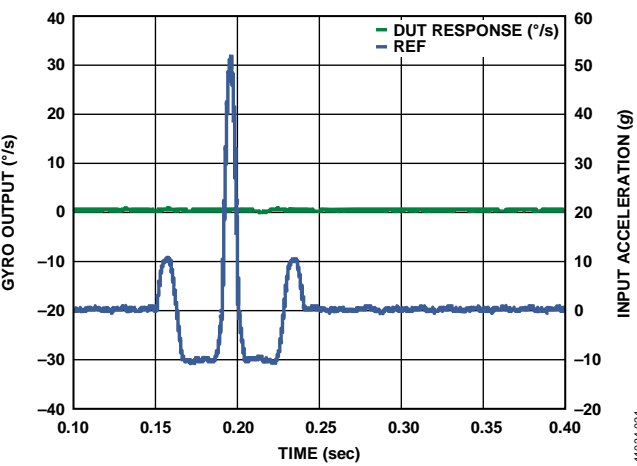
Figure 11. DUT Typical Response to 50 g, 10 ms Half-Sine Shock Test
