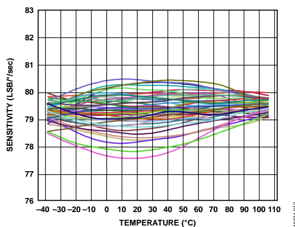
Figure 8. Sensitivity over Temperature (N > 100)
