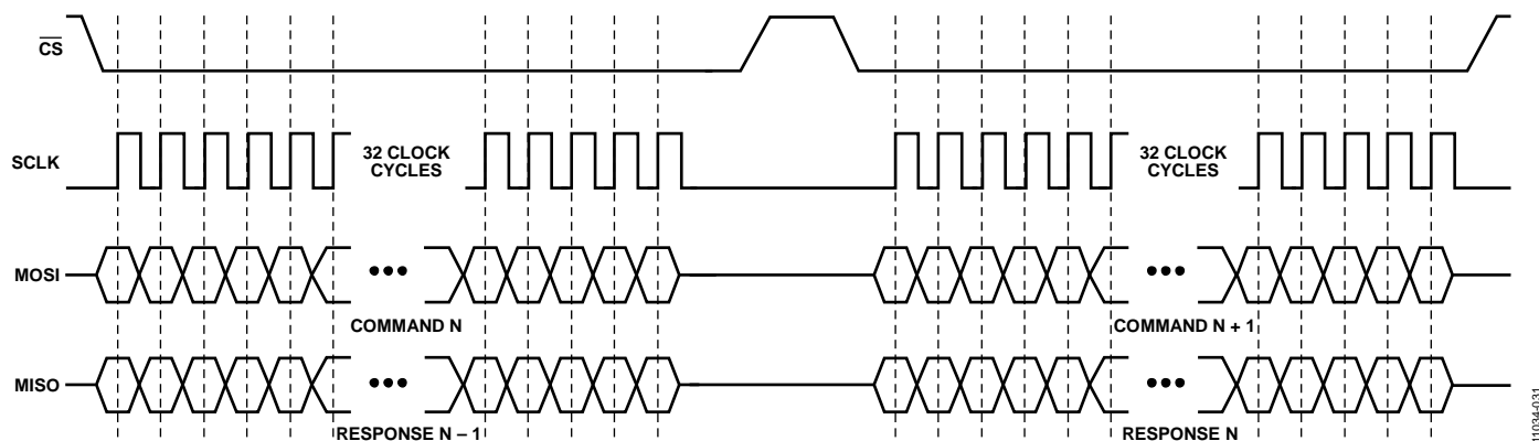
Figure 20. SPI Protocol
