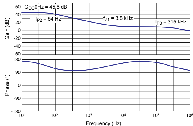
Figure 26. Compensated error amplifier Bode plot (SW3)
