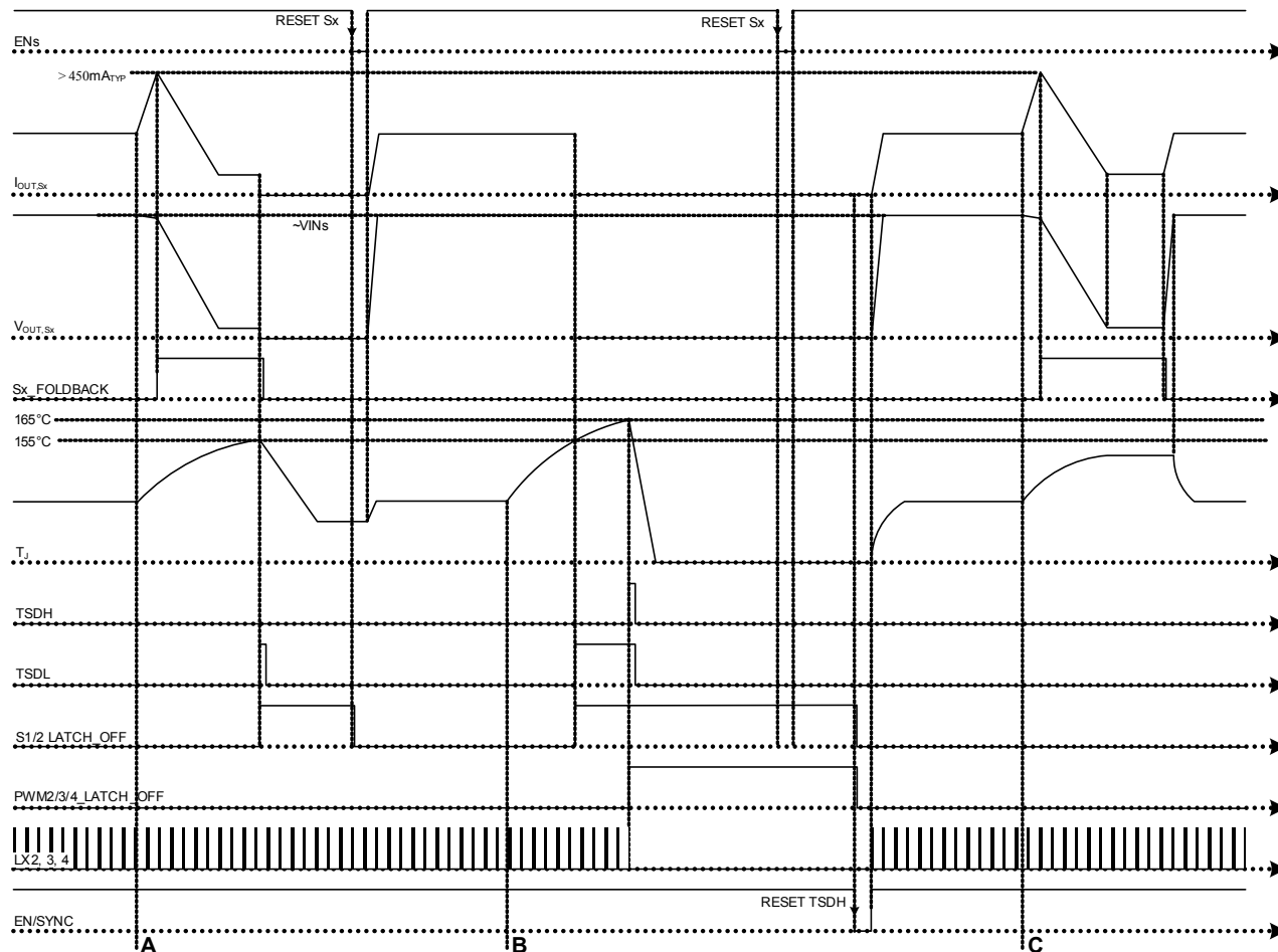
Figure 7. S1 and S2 Timing
