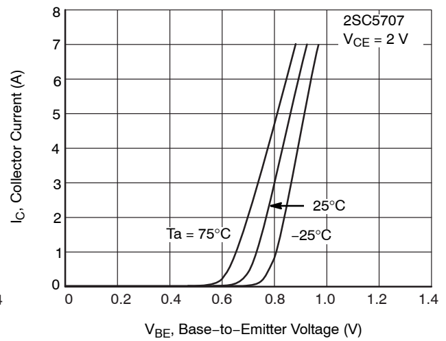
Figure 5. I_C - V_{BE}
