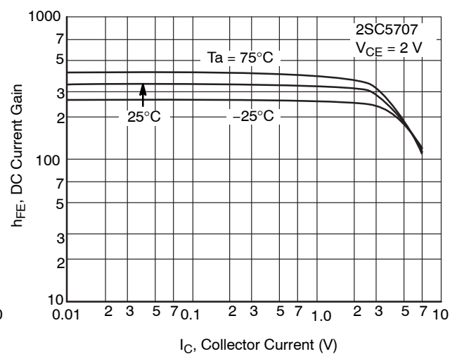
Figure 7. h_{FE} - I_C
