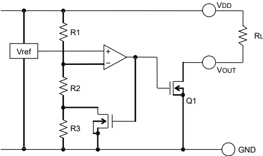
Fig.12 (BD48Exxx-M series Internal Block Diagram)
