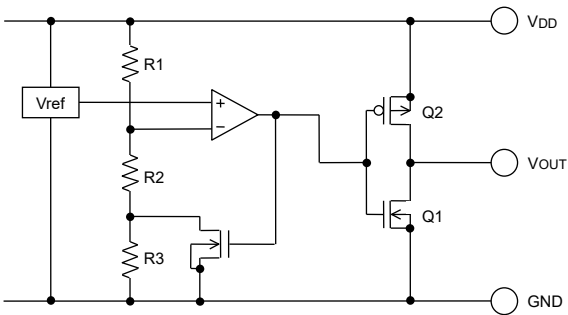
Fig.13 (BD49Exxx-M series Internal Block Diagram)
