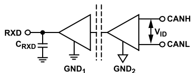
Figure 29. Receiver Voltage Measurement
