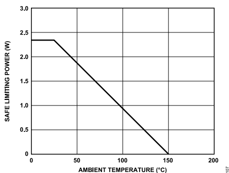
Figure 7. ADM3057E Thermal Derating Curve for 20-Lead Wide SOIC [SOIC_W] (RW-20) Package, Dependence of Safety Limiting Power with Ambient Temperature per IEC 60747-17
