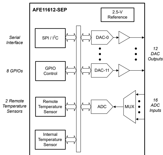
Simplified Schematic
