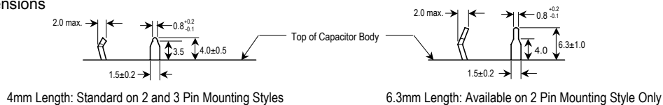
Pin Dimensions
