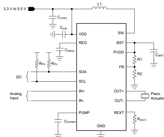
Simplified Schematic
