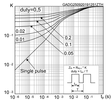
Figure 26. Thermal impedance for diode
