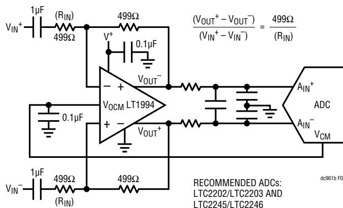
Figure 2. Typical Application for an LT1994
