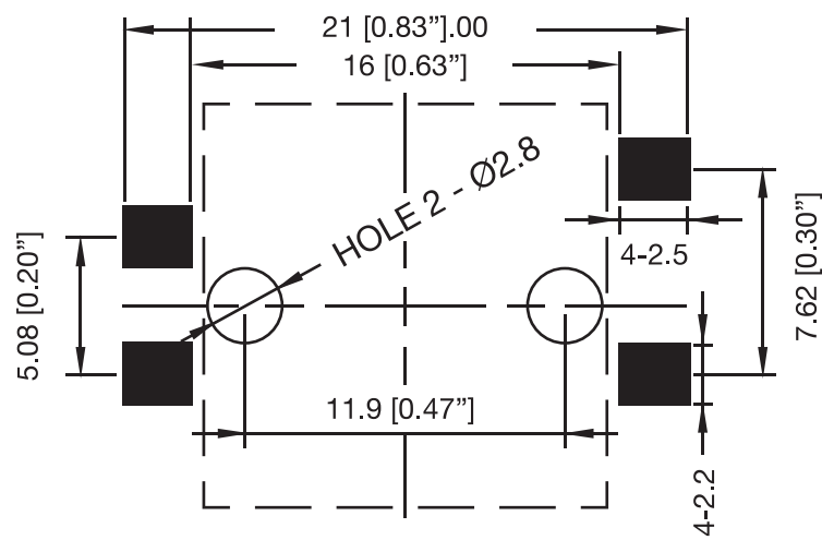
Top Mount
