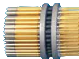
Planar Capacitor Array Diode Contacts
