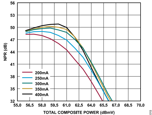
Figure 15. NPR vs. Total Composite Power Over Current, Worst Case Frequency, 10 dB Tilt, V_{DD} = 5.0 V
