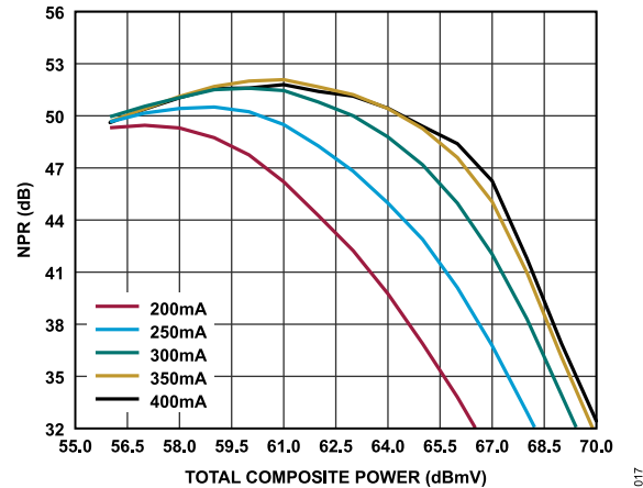
Figure 17. NPR vs. Total Composite Power Over Current, Worst Case Frequency, 10 dB Tilt, V_{DD} = 7.0 V
