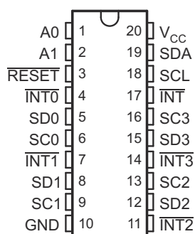
DG, DW, OR PW PACKAGE (TOP VIEW)
