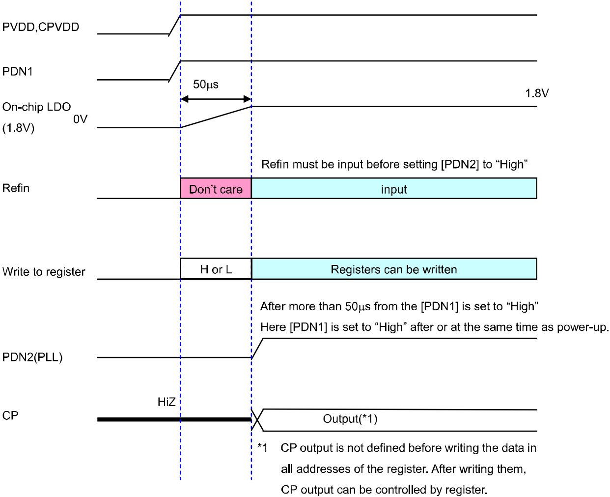
Fig. 13 Power Sequence
